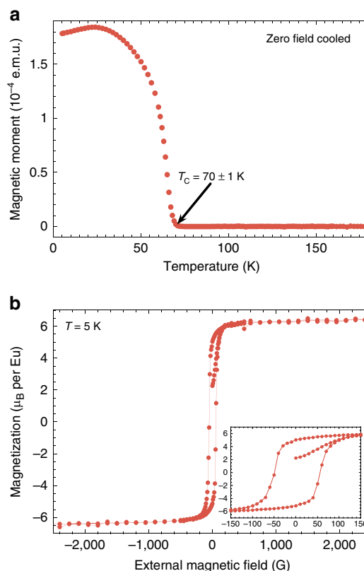
Figure 3 | Magnetic properties of topotactic \text{EuO} . (a) Spontaneous magnetization M(T) of an \text{EuO} film grown on (110) \text{YAlO}_3 via a topotactic transformation, measured using superconducting quantum interference device magnetometry in zero external field. Both the shape of the M(T) curve and the extracted T_C is typical of \text{EuO} films. The decrease of M(T) at low temperatures is due to domain effects. (b) M(\mu_0 H) curve of the same sample. The saturation magnetization of the film was determined to be 6.4_{-0.5}^{+0.8} \mu_B per Eu. The inset shows a magnified view of the hysteresis curve, which has a coercive field of 50 \pm 10 \text{ G} .
